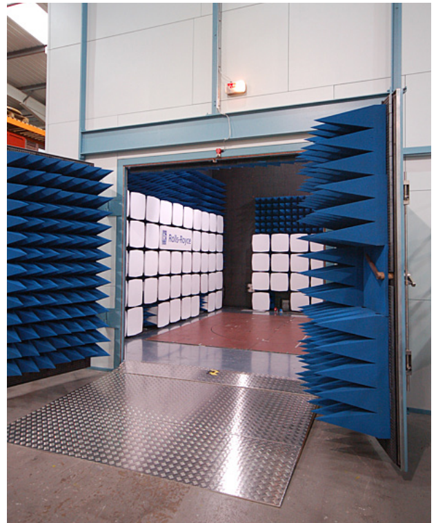
Low angle 2 stage removable ramps for forklift entry are available
